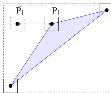
Figure 3.14: An oscillation of point P_1 between its current position and \tilde{P}_1 will throw events without any change in the hierarchy.
