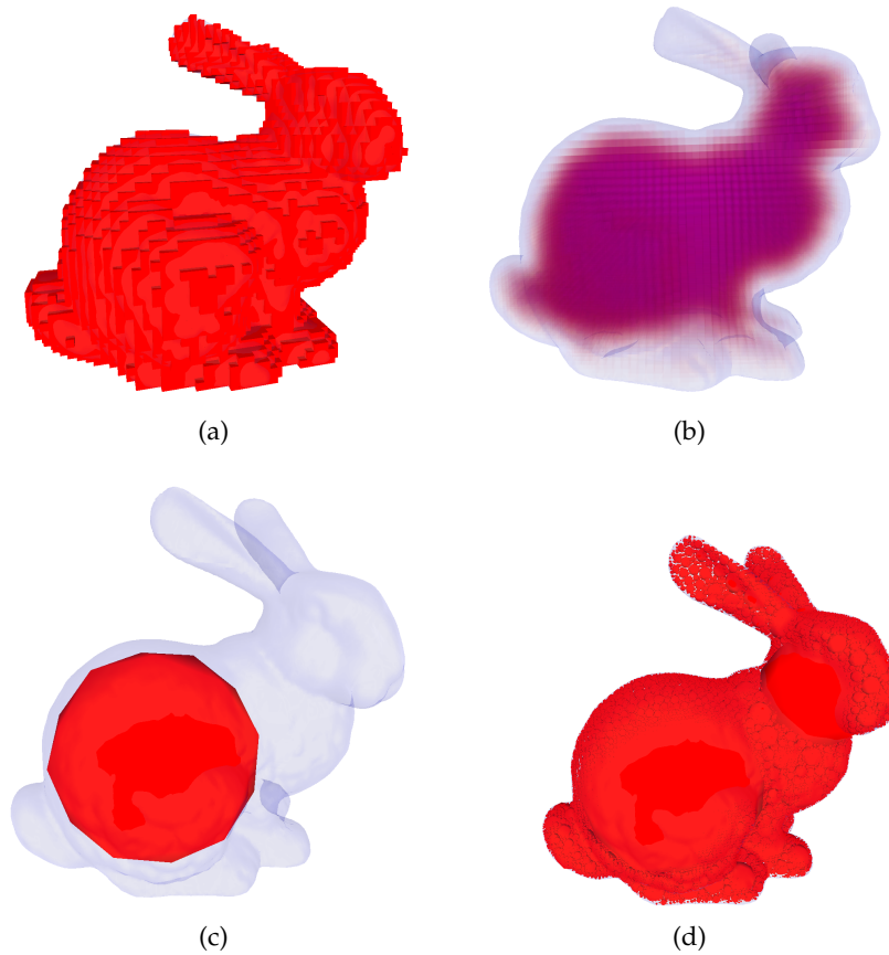
Figure 4.1: The different stages of our sphere packing algorithm: First, we voxelize the object (a) and compute distances from the voxels to the closest triangle ((b); transparency = distance). Then we pick the voxel with the largest distance and put a sphere at its center (c). We proceed incrementally and, eventually, we obtain a dense sphere packing of the object (d).
