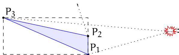
Figure 3.4: To keep the hierarchy valid when a leaf event happens, we have to replace the old maximum P_2 by the new maximum P_1 , and compute the time, when one of the other vertices of the polygon, P_2 or P_3 will become larger than P_1 . In this example this will be P_3 .
