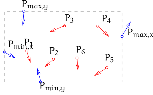
Figure 3.1: Assume a set of moving points in the plane. P_{\{\max,\min\},\{x,y\}} for the current bounding volume of this points. At some time, P_5 will become smaller than P_{\min,y} , this causes an event.
