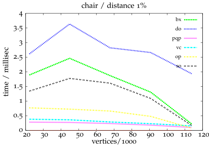
Figure 6.28: The dependency of the collision detection time from the complexity of the models in the chair scene. Again, the distance is fixed to 1% of the object size. In contrast to the castle scene (see Figure 6.27), the collision detection time decreases with an increasing complexity.
