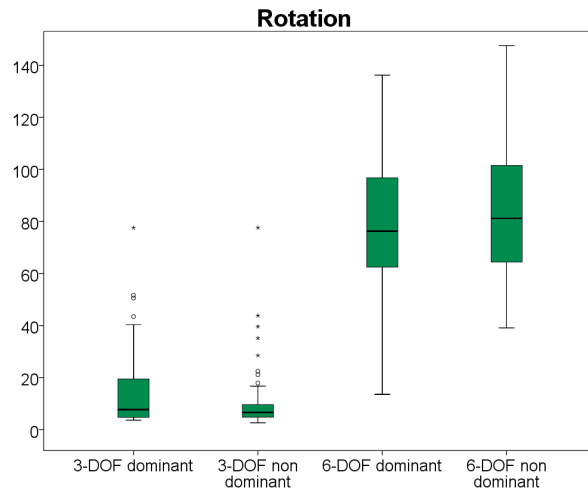
Figure 7.26: The total amount of rotations applied by the users during the game, which was obtained by accumulating the changes of the Euler angles. Obviously, the 3 DOF users avoid to rotate their virtual hands, probably because the orientation of the virtual hands is mapped to the buttons of the end-effector of the force-feedback device. (Usually, they brought it in a comfortable position during the training phase and did not change it during the game.
