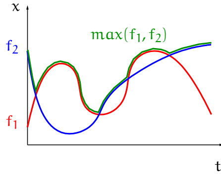
Figure 3.6: The flightplans are functions f_1 (red) and f_2 (blue) in the xt -plane and similarly in the yt - and zt -planes. The function \max(f_1, f_2) (green) determines the upper envelope of f_1 and f_2 .
