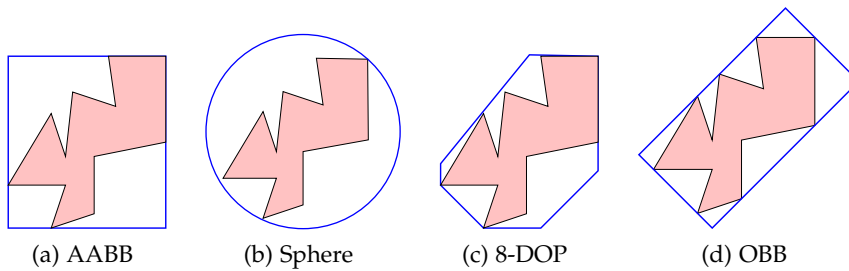
Figure 2.2: Different bounding volumes
