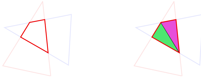
Figure 5.18: Our tetrahedron intersection method: the second step we tetrahedralize the resulting polyhedron.
