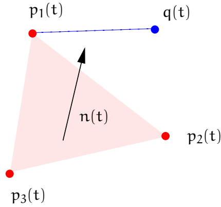
Figure 3.21: Continuous vertex/face-test: As a pre-condition of an intersection, q(t) has to be located in the triangles plane, i. e. (q(t) - p_1(t)) \cdot n(t) = 0 .
