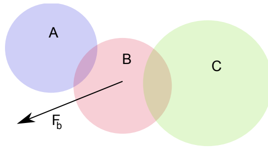
Figure 7.1: Sphere B has two adjacent spheres A and C. The penetration volume will be transferred to A, because A is closest to the direction of the force vector F_b .
