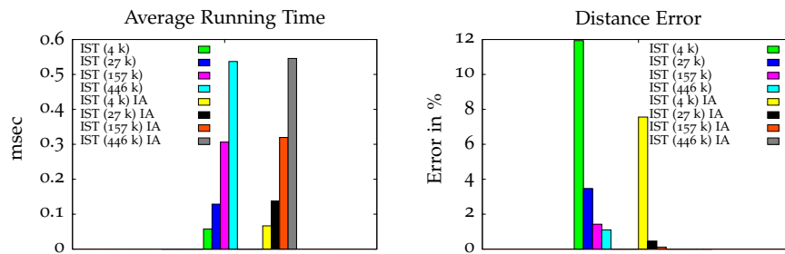
Figure 5.26: Pig scene: average and maximum time/frame (Left), relative error compared to accurate penetration volume (Right).
