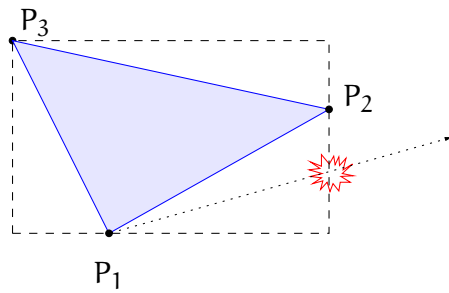
Figure 3.2: When P_1 becomes larger than the current maximum vertex P_2 , a leaf event will happen.
