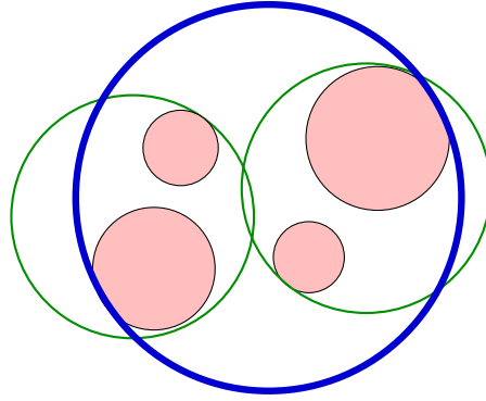
Figure 5.1: In a wrapped hierarchy, the blue sphere covers all its leaf nodes (red spheres), but not its direct children (green spheres).
