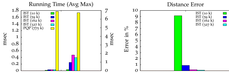
Figure 5.20: Oil pump scene: average and maximum time/frame (Left), relative error compared to accurate distance (Right).
