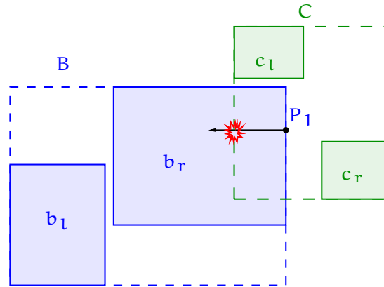
Figure 3.17: Fathers-do-not-overlap event: Currently, the BV pairs (b_l, c_l) , (b_l, c_r) , (b_r, c_l) and (b_r, c_r) are in the separation list. If their father BVs B and C do not overlap anymore, e. g. because the point P_1 that realizes the maximum of B becomes smaller than the minimum of C, we get an fathers-do-not-overlap event .
