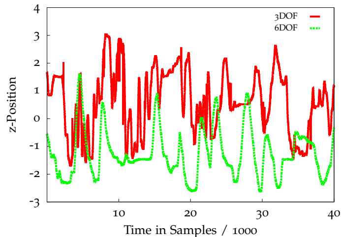
Figure 7.23: Typical data recorded from the users' interaction during the game. This plot shows the position of the haptic handle in z direction, which is controlled by the users' dominant hand with the 3 DOF (red) and 6 DOF device (green). Clearly, one can see the typical high frequencies caused by the "shovelling technique" that is often applied by 3 DOF users, whereas the 6 DOF users interact more precisely. Moreover, one can see how the 3 DOF user tries to distract the 6 DOF user at sample time 10k.
