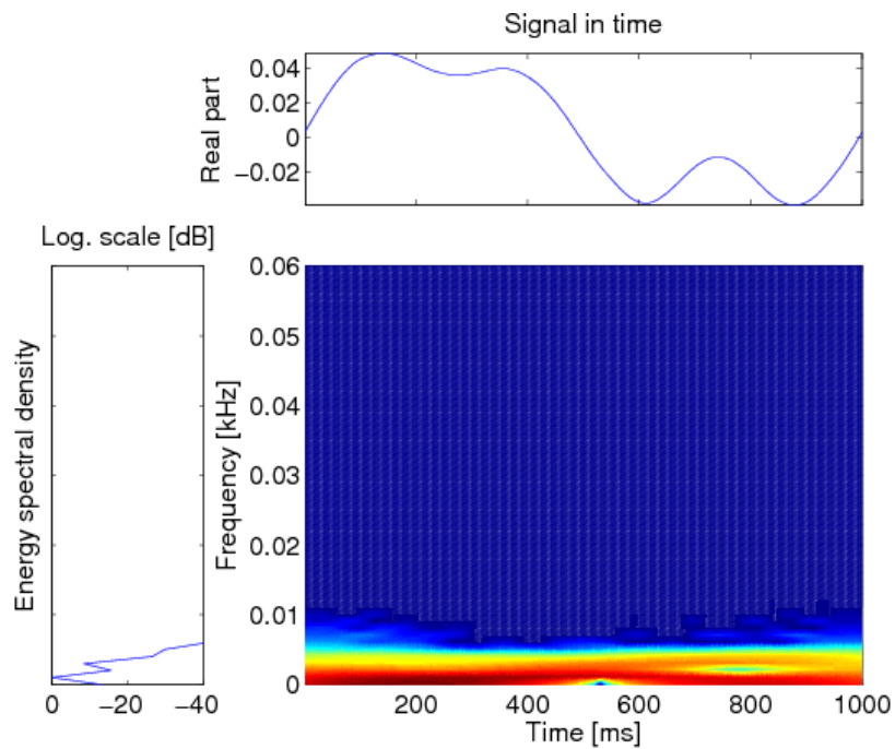
Figure 6.44: Noise in the force signal of the IST algorithm. Again, the colored picture shows the time frequency domain: the colors decode the intensity of the frequency, where dark blue remarks an intensity of zero.
