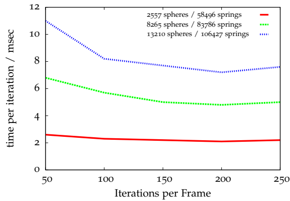
Figure 7.4: Average running-time of various sphere-spring systems with respect to the number of spheres and to the number of iterations.
