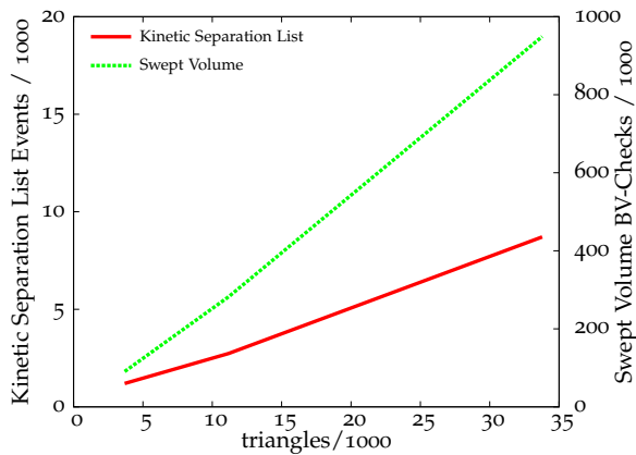
Figure 3.39: Swirling cloth scene: Number of events for the kinetic Separation-List and the number of collision checks for the swept AABB approach. Again, note the different scales.
