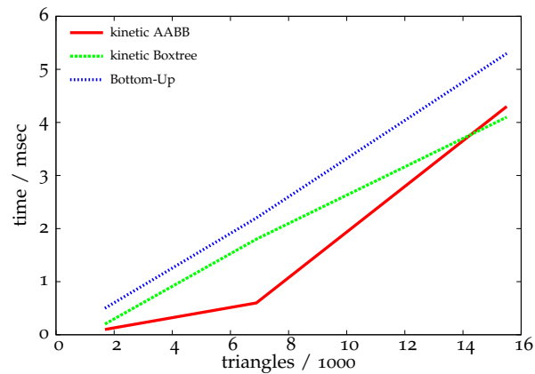
Figure 3.26: Tablecloth scene: Total time for updates and collision detection. Unfortunately, due to the relatively high deformation of the tablecloth and the high costs for the event-computation, the gain is lesser than expected, but there is still a significant gain for the kinetic AABB-Tree and the BoxTree.
