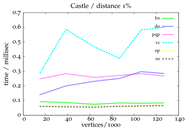
Figure 6.27: The dependency of the collision detection time from the complexity of the models in the castle scene. The distance is fixed to 1% of the object size. The collision detection time seems to be independent of the complexity.
