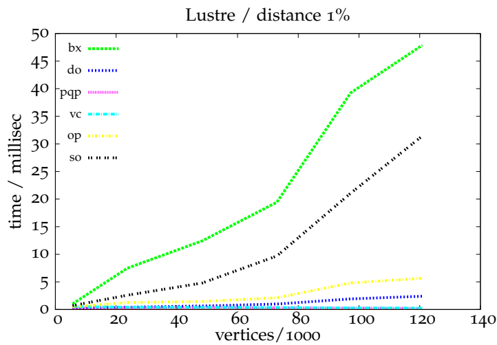
Figure 6.25: The results of the benchmark for the lustre scene for a distance of 1% relative to the object size. The x-axis denotes the number of vertices divided by 1000. The time for collision detection in this scene increases nearly linearly for the AABB-based algorithms.
