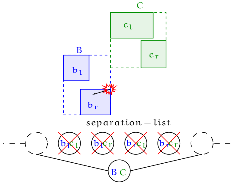
Figure 3.18: If a fathers-do-not-overlap event happens, that means B and C do not overlap anymore, we have to remove their child BVs (b_l, c_l) , (b_l, c_r) , (b_r, c_l) and (b_r, c_r) from the separation list and insert the new node (B, C) instead.
