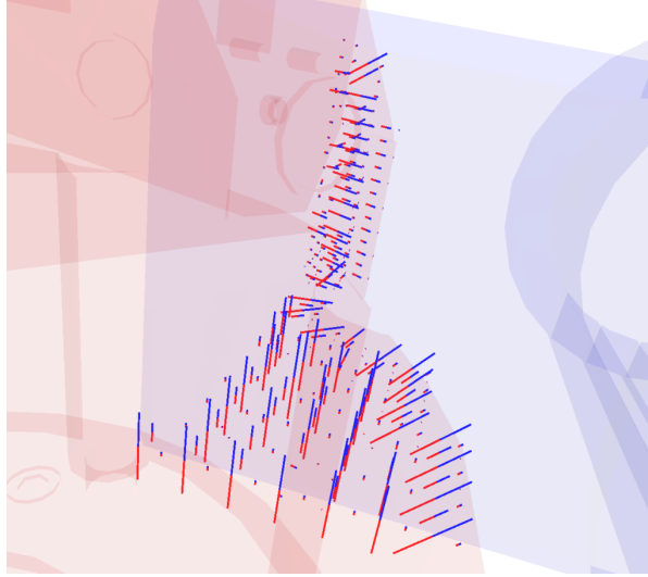
Figure 5.16: This image shows the normals for each pair of spheres overlapping each other, computed by our collision response scheme.
