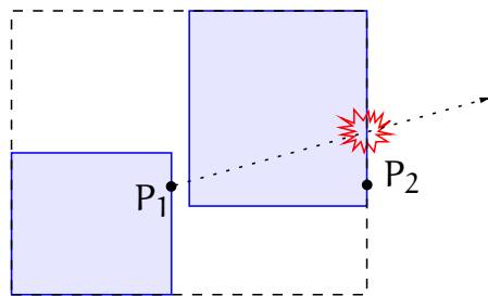
Figure 3.3: When P_1 , the maximum of the left child-box becomes larger than the overall maximum vertex P_2 , a tree event will happen.
