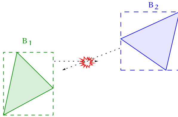
Figure 3.16: BV-overlap event: If the BVs B_1 and B_2 move so that they begin to overlap, we get an BV-overlap event .
