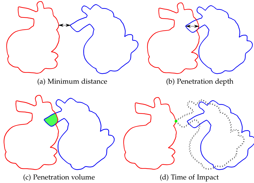
Figure 1.2: Different penetration measures.
