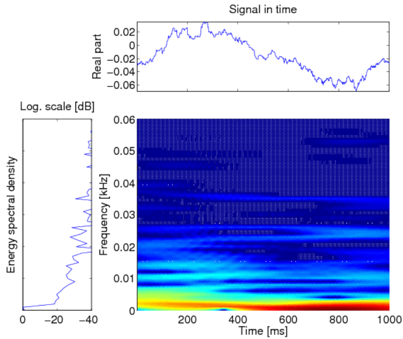
Figure 6.43: Noise in the force signal of the VPS algorithm. The colored picture shows the time frequency domain: the colors decode the intensity of the frequency, where dark blue remarks an intensity of zero.
