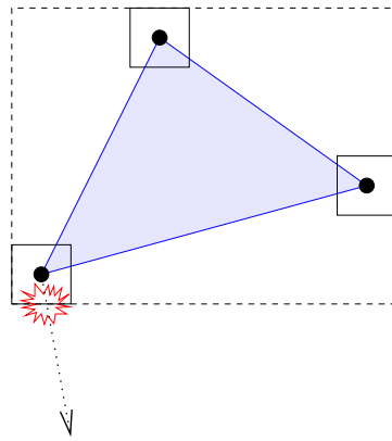
Figure 3.12: A point event happens if a point leaves its enclosing inflated BV.
