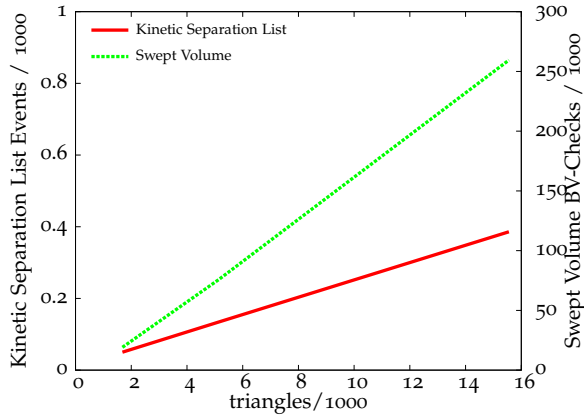
Figure 3.37: Tablecloth scene: Number of events in our kinetic data structure compared to the number of collision checks we have to perform with the swept-volume algorithm. The number of events is significantly smaller. Note the different scales.
