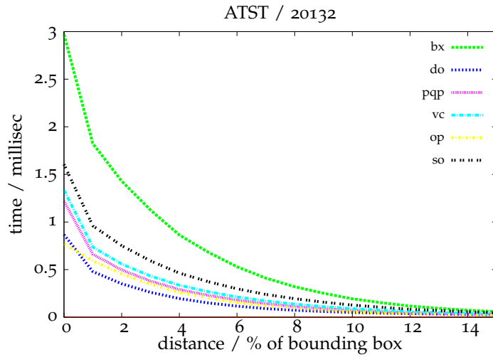
Figure 6.24: The results of the benchmark for the ATST walker with 20132 vertices. Like in the Apollo case (Figure 6.23), the OBB-based algorithms are much faster than the AABB-based libraries.
