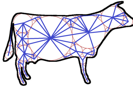
Figure 4.14: Our Protosphere algorithm does not only compute a sphere packing, but also maintains automatically the adjacency between the spheres, the so called Sphere Graph .
