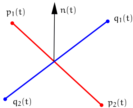
Figure 3.22: Continuous edge/edge-test: As a pre-condition of an intersection, both lines (p_1(t), p_2(t)) and (q_1(t), q_2(t)) have to be located in the same plane.
