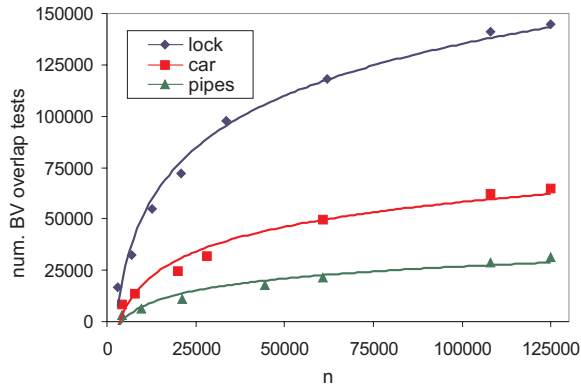
Figure 6.6: The number of visited BVTT nodes for models shown in Fig. 6.5 at distance \delta = 0.4 .
