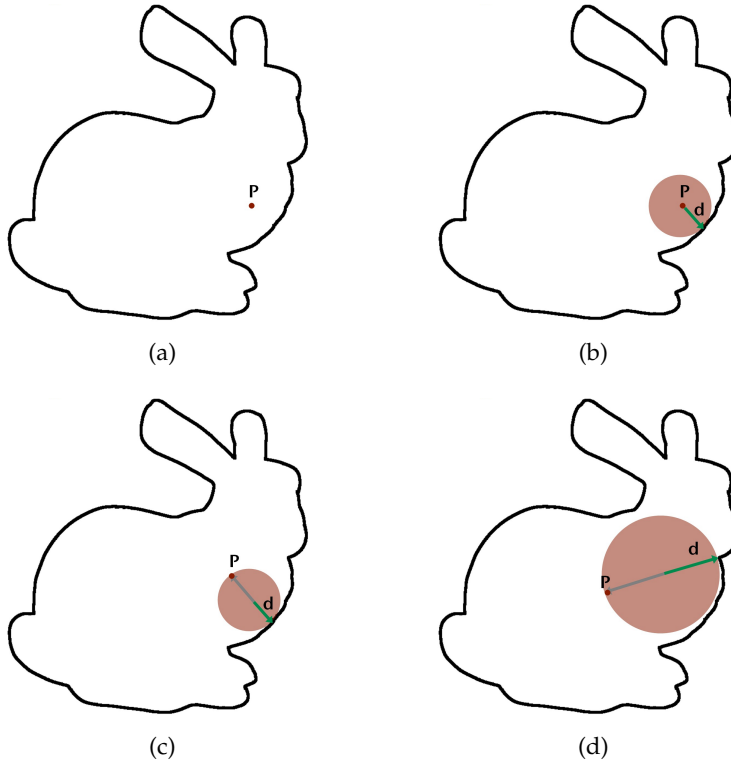
Figure 4.6: The prototype convergence algorithm: Place prototype P randomly inside the object (a). Compute minimum distance d from the prototype P to the surface (b). Move prototype P into the opposite direction, away from the surface (c) Continue until the prototype converges (d).
