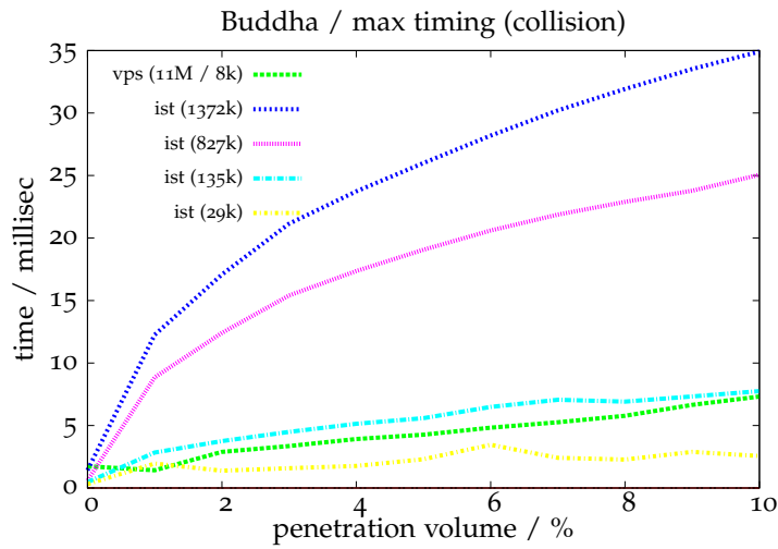
Figure 6.30: Scenario II, maximum running-time in the happy buddha scene
