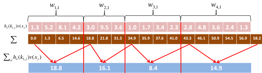
Figure 5.5: In order to compute the new position of the prototypes for the next iteration, we have to determine \sum h_\lambda(k_{ij})v(x_j)x_j . Therefore, we compute the prefix sum (brown array) for each of the four prototype arrays from Figure 5.4. The differences between the values at the borders directly deliver us the individual sum for each prototype.
