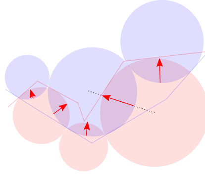
Figure 5.11: The direction of the penalty force can be derived from the weighted average of all vectors between the centers of colliding pairs of spheres, weighted by their overlap.
