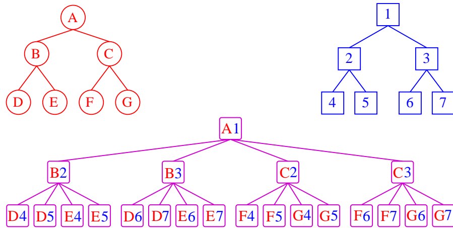
Figure 2.4: The simultaneous recursive traversal of two BVHs (red and blue) during the collision check results in a bounding volume test tree (purple).
