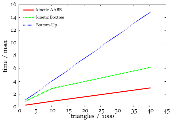
Figure 3.27: Expanding spheres scene: Average total time for the updates and the collision checks. This scene seems to be more appropriate for the KDSs than the tablecloth scene, despite the high amount of flightplan updates. The gain of the kinetic data structures compared to the bottom-up approach is more than a factor of five.
