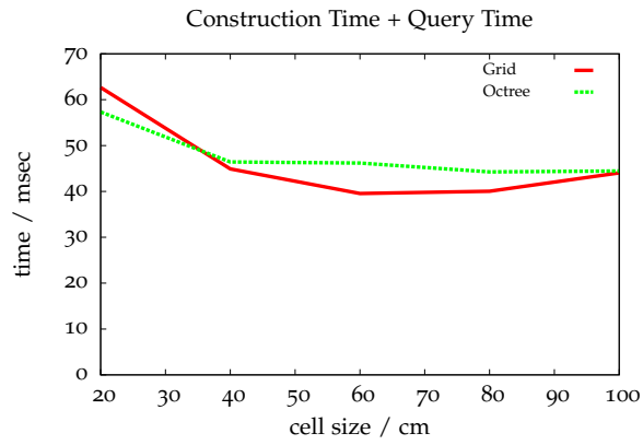
Figure 7.13: Combined construction and query time from Figures 7.11 and 7.12
