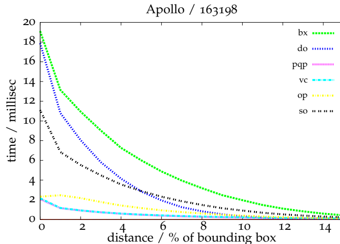
Figure 6.23: The results of the benchmark for the Apollo capsule with 163 198. In these test cases, the OBB-based algorithms are much faster than the AABB-based libraries.
