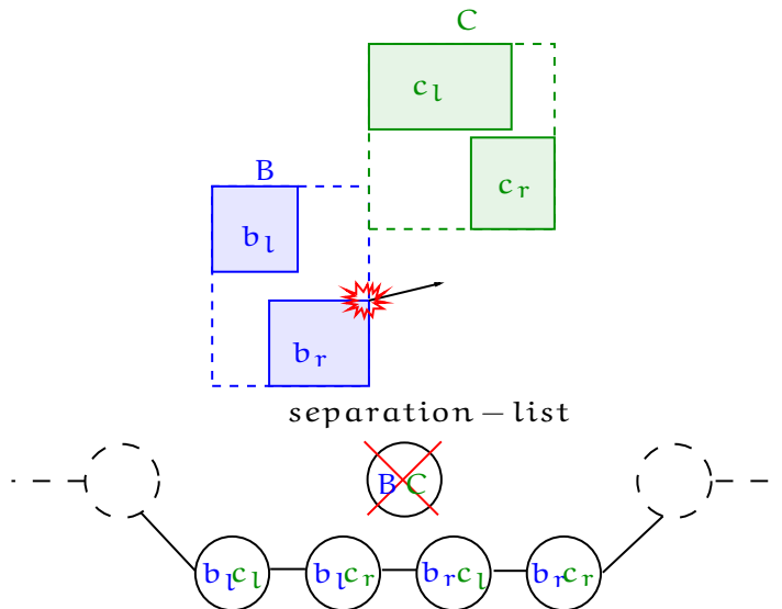
Figure 3.20: The BV-overlap event is somewhat the opposite of the fathers-do-not-overlap event (see Figure 3.18): If the BVs B and C begin to overlap, we have to remove the corresponding node from the separation list and insert their child BVs (b_l, c_l) , (b_l, c_r) , (b_r, c_l) and (b_r, c_r) instead.
