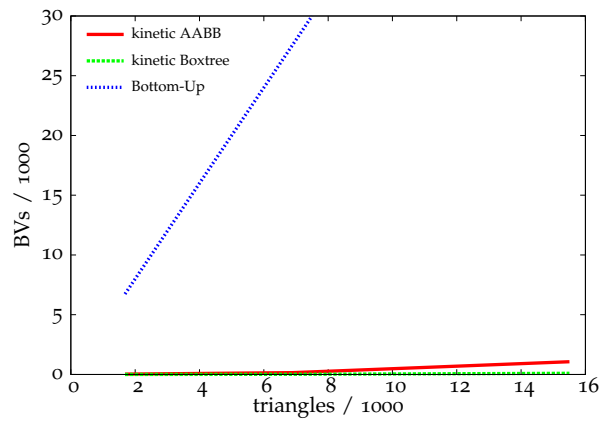
Figure 3.25: Tablecloth scene: The total number of updates is significantly smaller than the updates required by the bottom-up-strategy.
