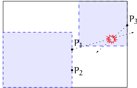
Figure 3.5: In case of a tree- and a leaf event, we have to propagate the change to upper BVs in the hierarchy. After replacing the old maximum P_2 by the new maximum P_1 in the lower left box, we have to compute the event between P_1 and P_3 , which is the maximum of the father.
