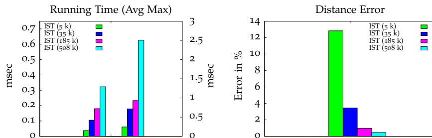
Figure 5.21: Armadillo scene: average and maximum time/frame (Left), relative error compared to accurate distance (Right).
