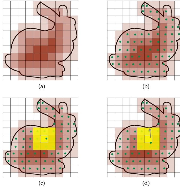
Figure 4.9: The parallel Protosphere algorithm: We use a discrete distance field. The discrete distance to the surface is colour coded (a). We place a prototype in each cell of the distance field (b). We use the discrete distance only to define a region in which we have to look for closest objects for each prototype (c). During the convergence step we clamp the prototypes to their cells (d).
