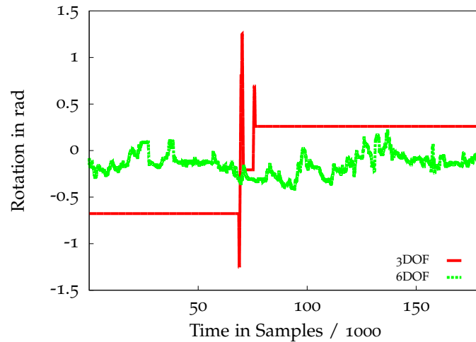
Figure 7.25: This plot shows the roll-angle of the 3 DOF (red) and the 6 DOF (green) users. The 6 DOF users typically rotate their virtual hands continuously, while the 3 DOF users let their hands in almost the same orientation at all times.
