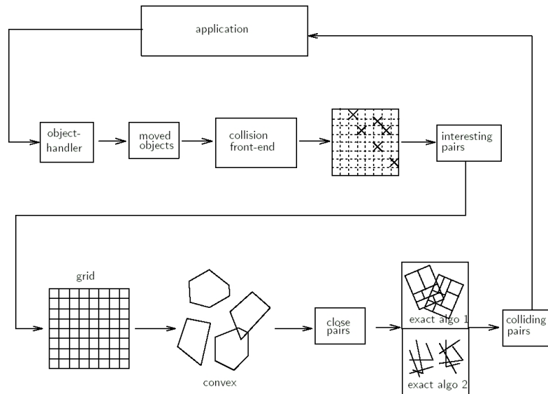
Figure 2.1: The typical design of a collision detection pipeline.
