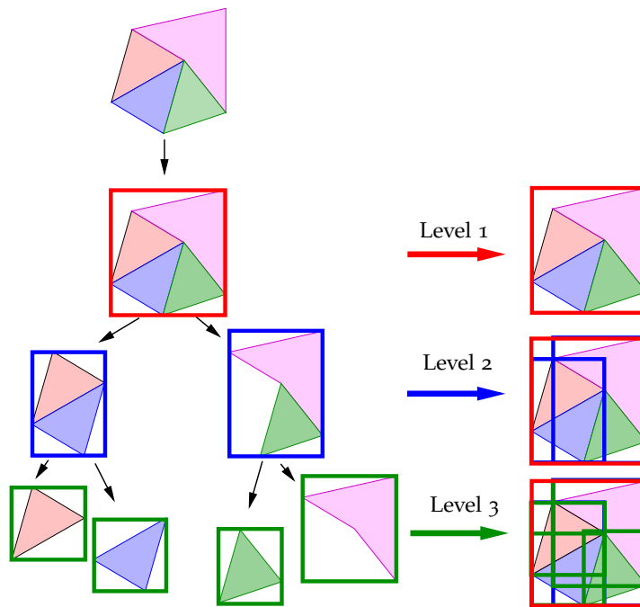
Figure 2.3: The BVH principle: Geometric objects are divided recursively into subsets of their geometric primitives (left) and each node on the tree realizes a bounding volume for all primitives in its sub-tree (right).
