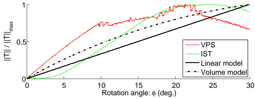
Figure 6.40: Torques in Scenario III.
