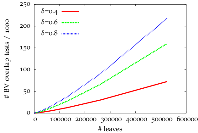
Figure 6.9: The asymptotic number of overlapping BVs depends mainly on \alpha , the BV diminishing factor, and only to a minor extent on \delta , the penetration depth of the root BVs. In this plot \alpha = 0.6 .
