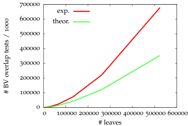
Figure 6.8: Same as Plot 6.7 but with \alpha = 0.9 .
