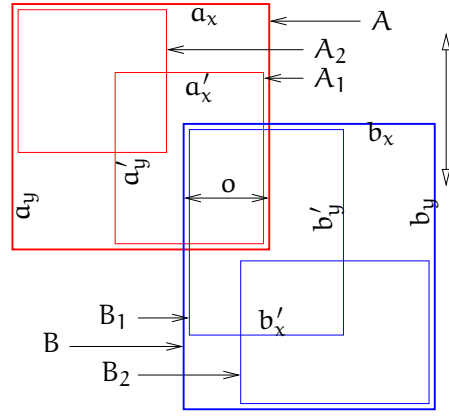
Figure 6.1: General configuration of the boxes, assumed throughout our probability derivations. For sake of clarity, boxes are not placed flush with each other
