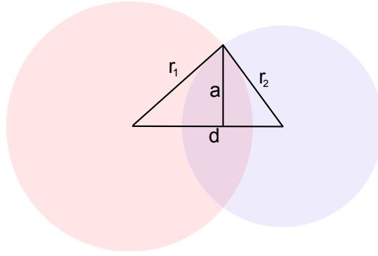
Figure 5.6: Penetration volume of two spheres with radius r_1 and r_2 , respectively.
