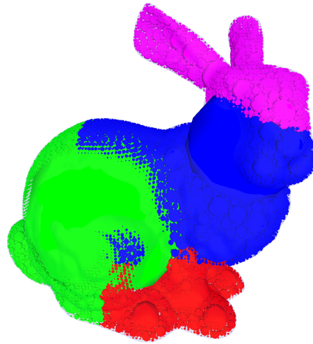
Figure 4.3: An object filled with the voxel-based sphere packing method. On the body, you can see the regular spheres that were produced due to the fixed center positions.
