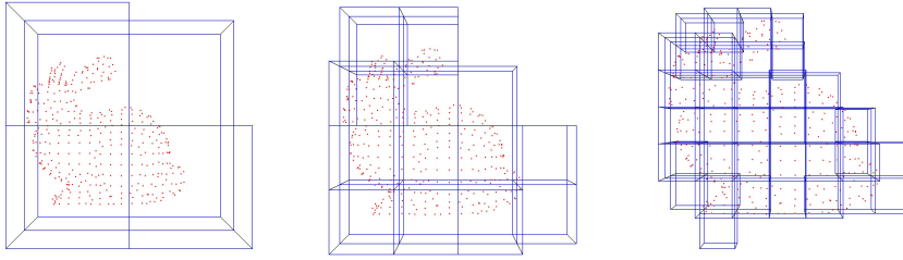
Figure 7.9: Different octree levels for a point cloud model of a bunny.
