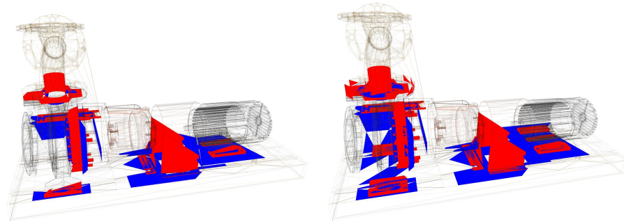
Figure 6.45: The intersecting triangles that were found by PQP (left) and CollDet (right) in a typical CAD simulation. You can see, that CollDet finds much more intersecting triangles.
