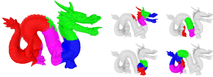
Figure 5.2: This figure shows the results of our hierarchy building algorithm based on batch neural gas clustering with magnification control. All of those inner spheres that share the same color are assigned to the same bounding sphere. The left image shows the clustering result of the root sphere, the right images the partitioning of its four children.
