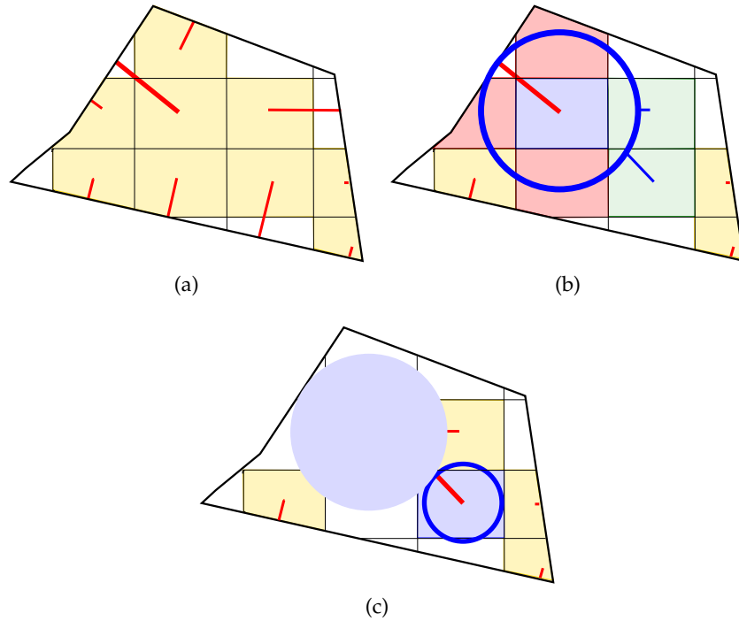
Figure 4.2: This figure shows the first steps of the creation of the inner spheres. First, the object is voxelized (a). Additionally, we compute the shortest distance to the surface (red lines) for interior voxel centers (yellow), i. e. a discretization of the interior distance field. Next, we place a maximal sphere at the voxel center with the largest radius (blue sphere). Then those voxels whose centers are located inside the new sphere (red), are deleted, and the shortest distances of some voxels are updated, because they are now closer to the new inner sphere (green)(b). This procedure continues greedily (c).
