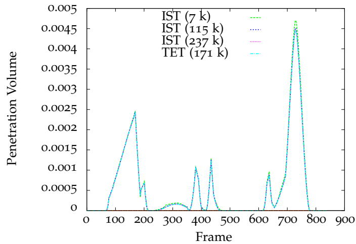
Figure 5.25: Penetration volume per frame in the bolt scene.
