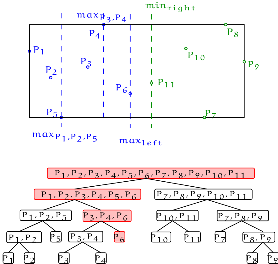
Figure 3.8: In order to compute a new event for \max_{\text{left}} , we have to look which vertex can become larger than \max_{\text{left}} that is recently realized with P_6 . In the first level, this could be either the maximum of the left sub-tree, the vertex P_5 , or any vertex in the right sub-tree of node (P_1, P_2, P_3, P_4, P_5, P_6) . On the next level it could be the maximum of the left sub-tree of node (P_3, P_4, P_6) , thus the vertex P_4 , and all vertices in the right sub-tree, that only contains P_6 .
