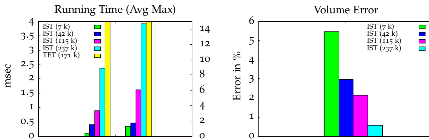
Figure 5.24: Bolt scene: average and maximum time/frame (Left), relative error compared to accurate penetration volume (Right).
