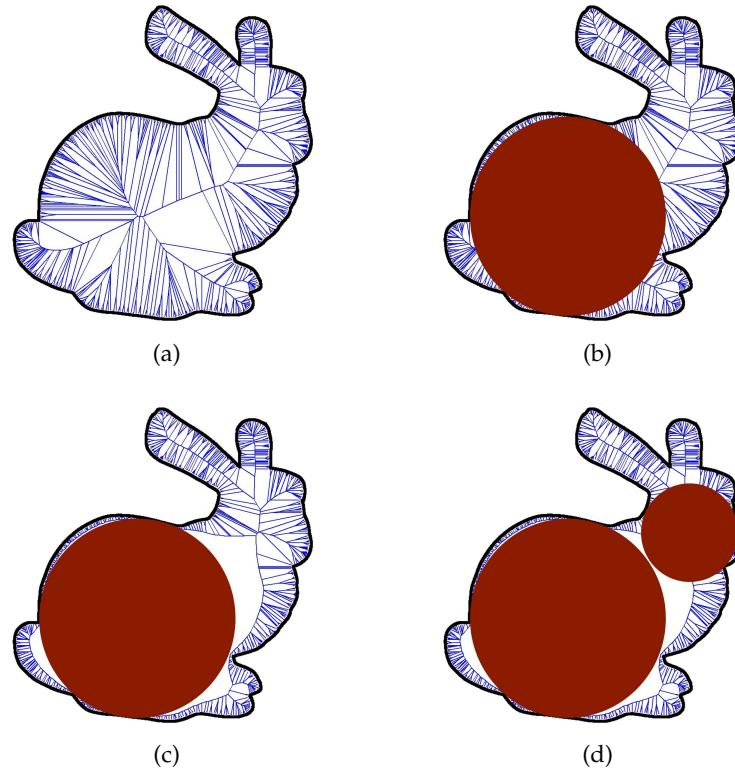
Figure 4.5: The basic idea of our Protosphere algorithm: compute a Voronoi diagram for the object (a), place the largest sphere (b), recompute Voronoi diagram for the object and the new sphere (c), place largest sphere in the new Voronoi diagram etc. (d).
