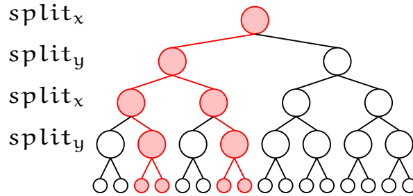
Figure 3.9: If more than one splitting axis are allowed, we have to search for the next level with the same splitting axis, when we want to look for the next candidates for an event. We have to visit the red marked nodes when we compute a new event for the root box.
