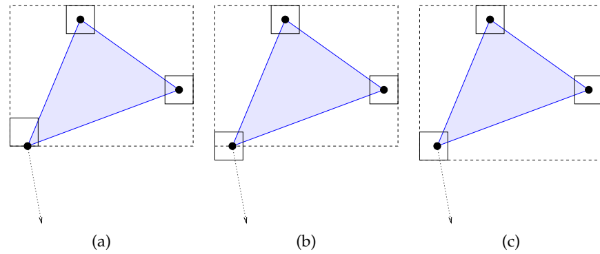
Figure 3.13: When a point event happens (a), we move the into the appropriate direction (b) and recompute the BV (c). Moreover, we have to propagate the change in the hierarchy.
