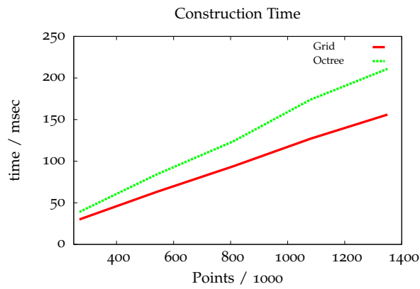
Figure 7.14: Average construction time for point clouds with respect to the size of the point cloud. The cell size was set to 8 cm.
