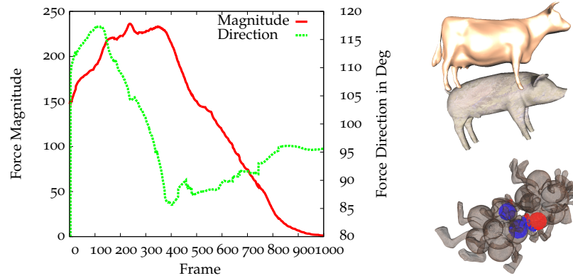
Figure 5.12: Left: force magnitude (red) and direction of the force vector (green) during the cow/pig animation. Right: the test scenes. A cow scraping alongside a pig (upper), two instances of a monster with complex extremities tangled up (lower).
