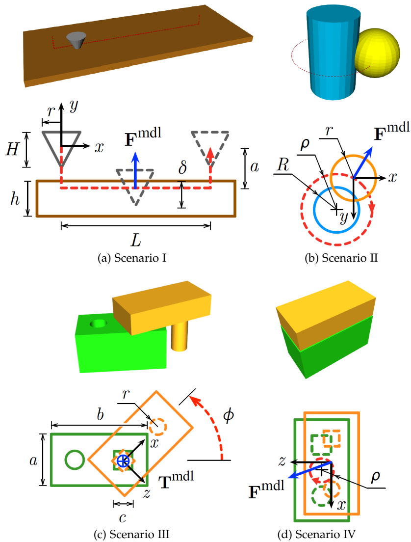
Figure 6.35: Scenarios in the force and torque quality benchmark as explained in Section 6.4.2. Upper row shows 3D snapshots, whereas the lower displays parametrized schematics. Trajectories are represented with red dashed curves. Expected relevant forces and/or torques are shown with blue vectors. Coordinate systems are placed in points where forces and torques are measured – for the cone and the sphere this point is in their AABB center, whereas the position in z axis for the "Pins" object is in the middle of the pin.
