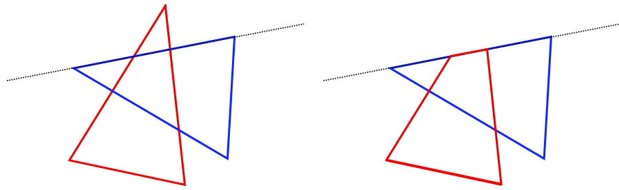
Figure 5.17: Our tetrahedron intersection method: in the first step, we clip the triangles of the red tetrahedron against the planes that span the blue one.
