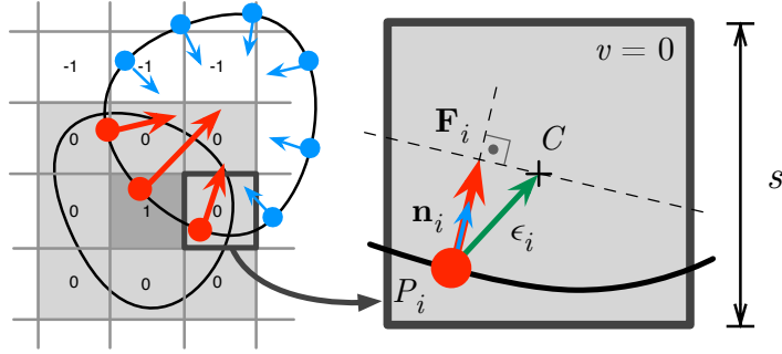
Figure 6.36: On the left, a layered voxmap (bottom) is colliding with red pointshell points (top), yielding red bold collision forces. On the right, the computation of a single collision force related to a colliding point is graphically shown. Single collision forces are computed scaling the normal vector ( n_i ) of the colliding point ( P_i ) with the sum of the local ( n_i \epsilon_i ) and global ( vs ) penetration of the point in the object.
