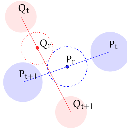
Figure 5.10: Determining the point of impact for a pair of spheres.
