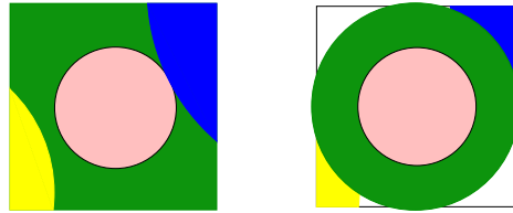
Figure 5.7: After constructing the sphere packing with the voxel-based method (see Section 4.2), each voxel can be intersected by several non-overlapping spheres (left). These do not necessarily account for the whole voxel space (green space in the left picture). In order to account for these voids, too, we simply increase the radius of the sphere (green sphere) that covers the center of the voxel (right).
