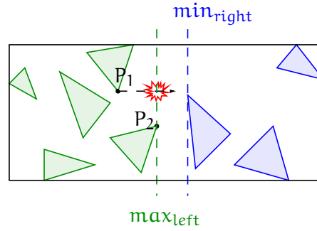
Figure 3.7: If a vertex in the left sub-tree becomes larger than the point P_2 that realizes its current maximum \max_{\text{left}} , a tree event will happen. Similarly, we get an event for the right sub-tree, if a point in it becomes smaller than its current minimum \min_{\text{right}} .
