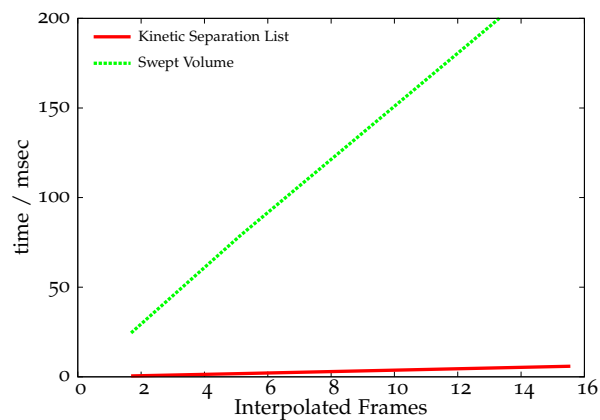
Figure 3.36: Tablecloth scene: Total time, this means updating the hierarchies and the time for the collision check including self collision. The gain of our kinetic data structures is about a factor of 50.
