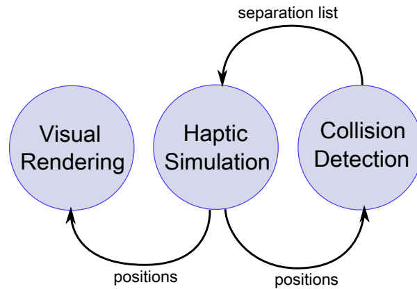
Figure 7.16: The simulation thread in our haptic workspace computes the collision forces based on the separation list , which captures the current collision information. This list is generated in the collision detection thread. Conversely, the haptic thread passes the new positions of the objects to the collision and the (visual) rendering thread.
