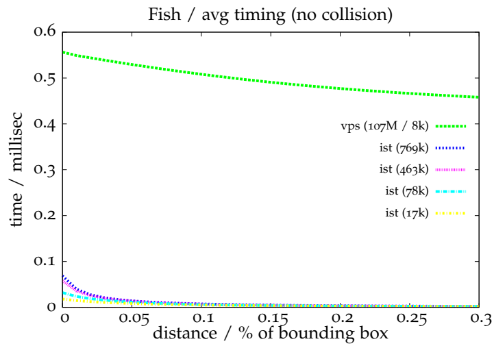
Figure 6.33: Scenario I with ISTs and VPS, average running-time in the fish scene
