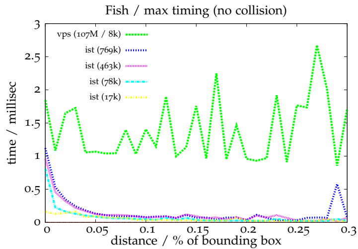
Figure 6.34: Scenario I with ISTs and VPS, maximum running-time in the fish scene
