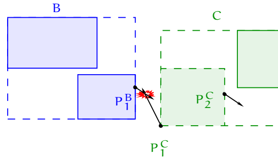
Figure 3.19: If the flightplan of P_2^C changes, this has no effect on the separation list, and thus, no BV-change event will happen due to this change.
