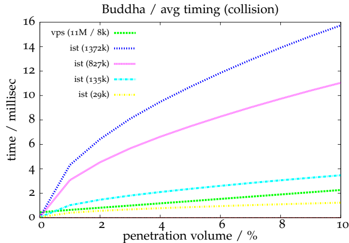
Figure 6.29: Scenario II, average running-time in the happy buddha scene: on the x-axis you find the amount of overlap in percent of the object's total volume. The number in parentheses after IST denotes the number of spheres in thousands. The two numbers after VPS denote the number of voxels and points in thousands, respectively.
