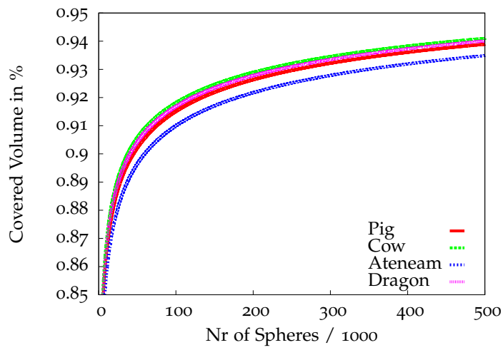
Figure 4.12: The space filling rate of our sphere packing algorithm.
