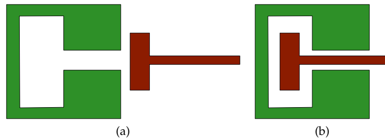
Figure 6.16: The sphere method will find only configuration (a) for the red and the green objects, but it will miss configuration (b).
