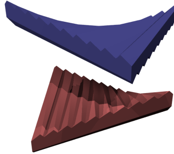
Figure 1.1: The intersection of two Chazelle polyhedra is a worst case for collision detection algorithms.
