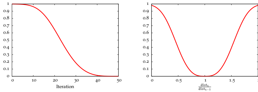
Figure 4.7: Plots of our cooling functions: \varepsilon(t) with t_{\max} = 50 and c = 5 (left). \varepsilon(d) with c = 2 (right).
