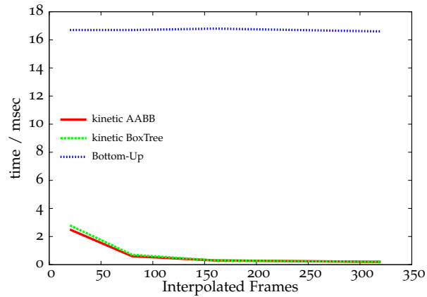
Figure 3.30: Male cloth animation scene: Average update time depending on the number of interpolated frames between two key frames. Since the number of events only depends on the number of key frames and not on the number of interpolated frames, so, the average update time decreases if we increase the total number of frames.
