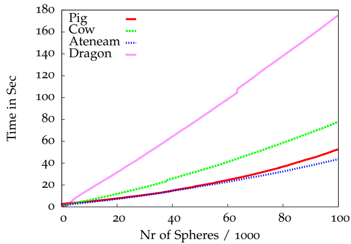
Figure 4.13: Timings for different objects on a Geforce GTX480 (right; please note that the code is not optimized yet).
