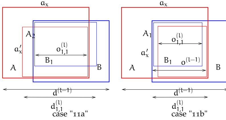
Figure 6.3: Denotations for computing d_{11}^{(l)} for a child pair. If a'_x > o^{(l-1)} , the new distance d_{11}^{(l)} is d_{i,j}^{(l-1)} - 2\omega^{(l)} with \omega^{(l)} = \alpha_x^{(0)} \alpha_x^0 (1 - \alpha_x) = \alpha_x^{(0)} (1 - \alpha_x) . In the other case, d_{11}^{(l)} equals the overlap o^{(l-1)} .
