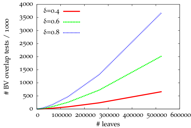
Figure 6.10: Same as Plot 6.9 with \alpha = 0.7
