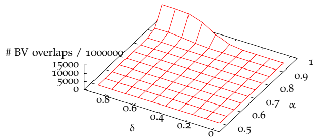
Figure 6.13: Same as Plot 6.12 but with n = 524288 leaves.
