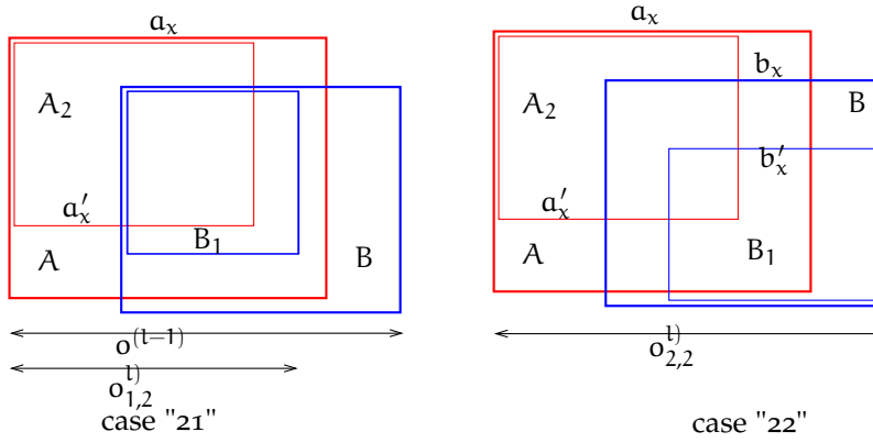
Figure 6.4: The case "12" is symmetric to "21", and the case "22" is trivial. Here, \omega^{(l)} = \alpha_x^{(0)} \alpha_x^0 (1 - \alpha_x) = \alpha_x^{(0)} (1 - \alpha_x) .
