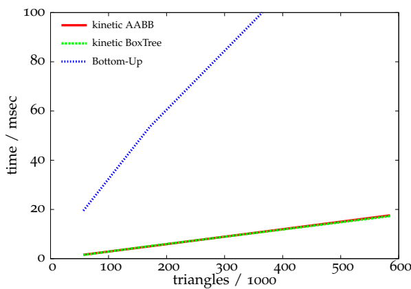
Figure 3.29: Catwalk scene: Updating times. In this scene we have an overall gain of a factor about 10 for the kinetic AABB-Tree compared to the bottom-up-update.
