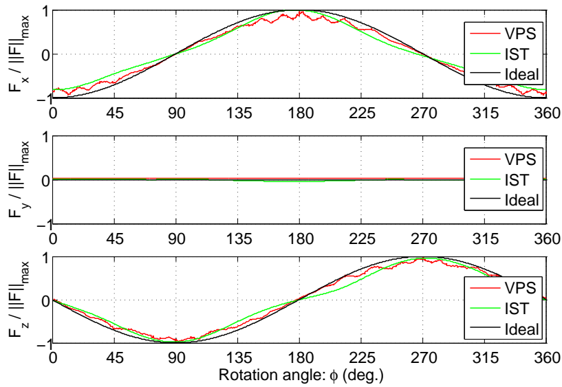
Figure 6.42: Forces in Scenario IV.
