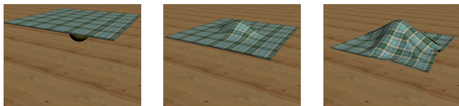
Figure 2.6: Deformable objects like cloth require special algorithms, because pre-computed data structures become invalid after the deformation. Moreover, collision between parts of the object itself may happen.
