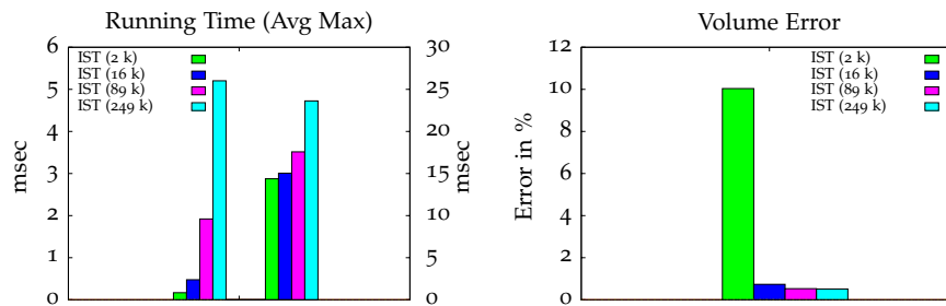
Figure 5.27: Screwdriver scene: average and maximum time/frame (Left), relative error compared to accurate penetration volume (Right).
