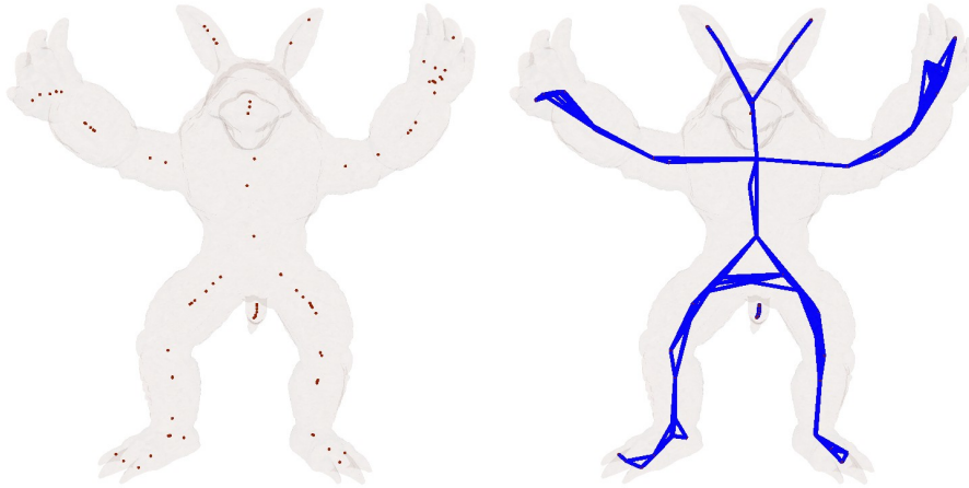
Figure 4.10: After the convergence of the initial prototypes, our parallel algorithm yields an approximation of the object's Voronoi nodes (left). If we connect overlapping spheres, we get an approximation of the medial axis (right).
