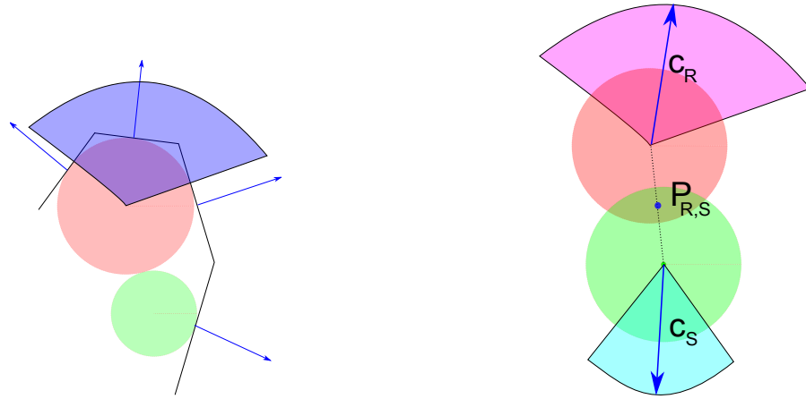
Figure 5.15: Left: we compute a normal cone for each inner sphere. The cone bounds a list of triangles that is associated with the sphere. Note that the spread angle of the normal cone can be 0 if the sphere is closest to a single triangle (e. g. the green sphere). Right: the axis of the normal cones c_R and c_S are used for the force direction. The center P_{R,S} of the spherical cap defines the contact point.
