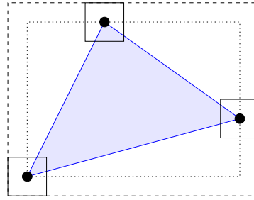
Figure 3.11: Kinetic Interval DOP: We inflate each point by a certain amount.
