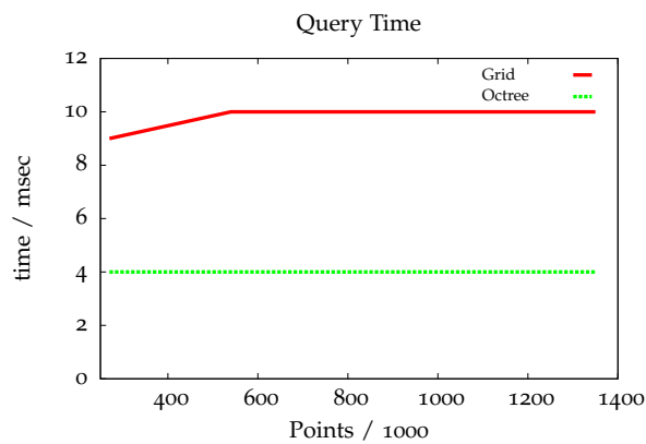
Figure 7.15: Average query time for point clouds with respect to the size of the point cloud. The cell size was set to 8 cm.
