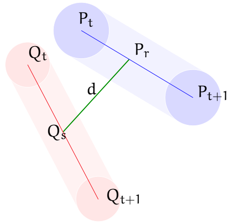
Figure 5.9: The centers of the blue and the red sphere move from position P_t to P_{t+1} , and Q_t to Q_{t+1} respectively, in a time step of the simulation. Spheres in deeper hierarchy levels can only collide, if the capped cylinders that are spanned by the moving spheres overlap. The intersection between the capped cylinders can be easily determined by computing the minimum distance d between the line segments (P_t, P_{t+1}) and (Q_t, Q_{t+1}) that is realized by the points P_r and Q_s .
