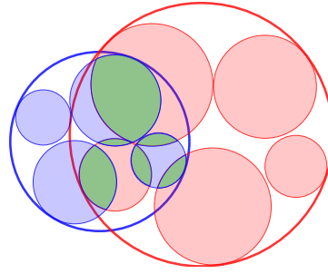
Figure 5.8: We estimate the real penetration volume (green) during our time-critical traversal by the “density” in the hierarchy spheres (blue and red) and the total volume of the leaf spheres.
