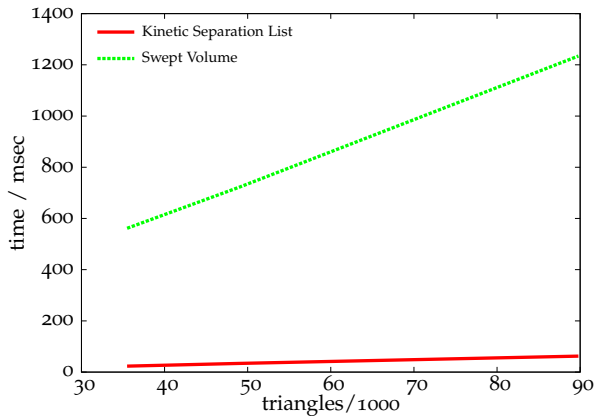
Figure 3.34: Male cloth animation scene: Average total time for updating the hierarchies and performing the inter- and intra-collision detection. We have an overall gain of about a factor of 20 with our kinetic Separation-List.
