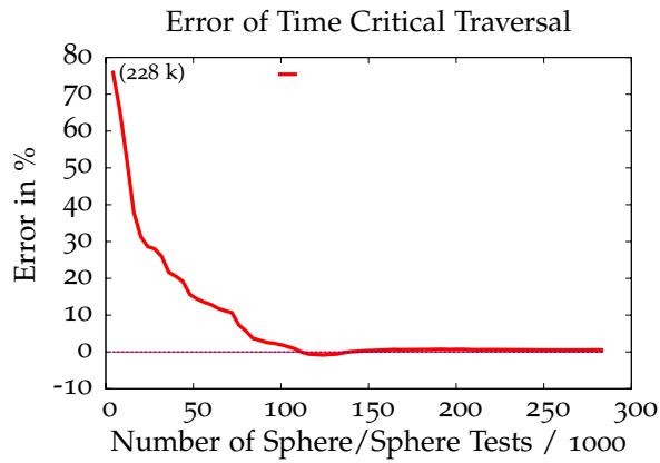
Figure 5.29: Error relative to the exact penetration volume depending on the number of intersection tests during time critical penetration volume computations in the torso scene
