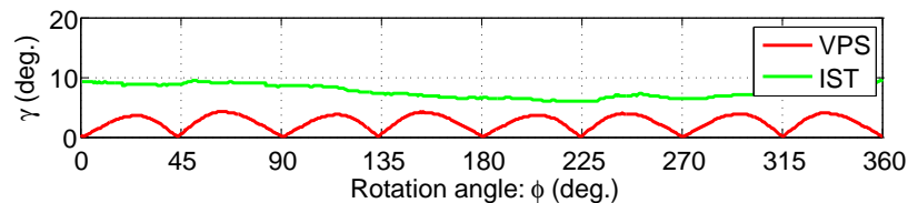
Figure 6.39: Average angle between analytical model and measured values in Scenario II.
