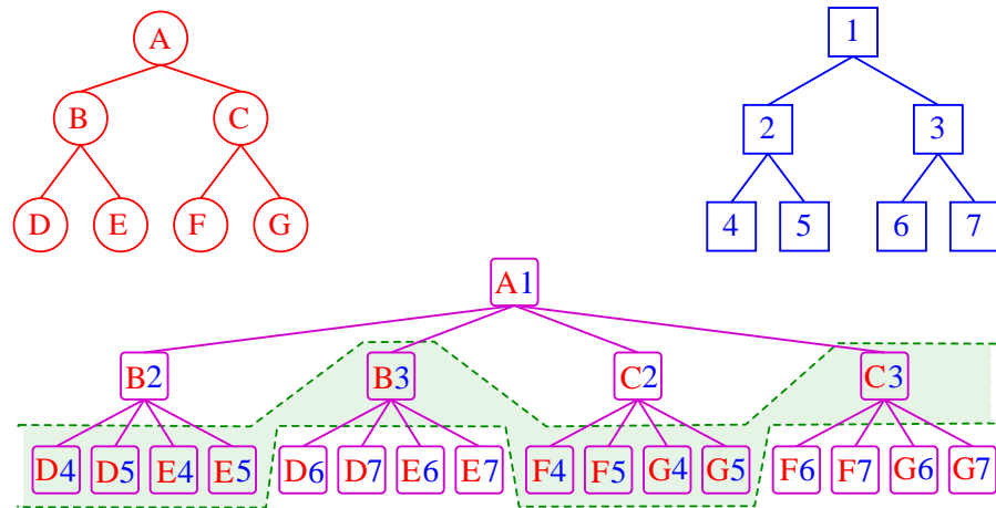
Figure 3.15: The simultaneous traversal of two BVHs results in a BVTT (see Figure 2.4). Those BV pairs, where the traversal stops, build a list in this tree (green). We call it the separation list . This list consists of inner nodes, whose BVs do not overlap (B, 3) and leaf nodes, where the BVs are leaves in the BVH that do either overlap or not.
