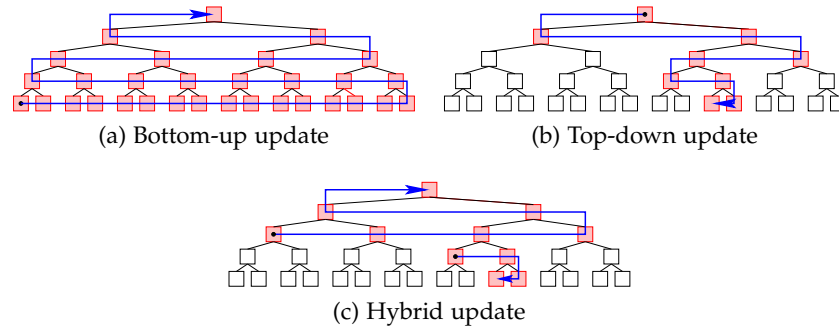
Figure 2.7: Different updating strategies for BVHs.
