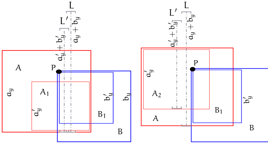
Figure 6.2: The ratio of the length of segments L and L' equals the probability of A_1 overlapping B_1 (left), and A_2 overlapping B_1 (right), respectively.
