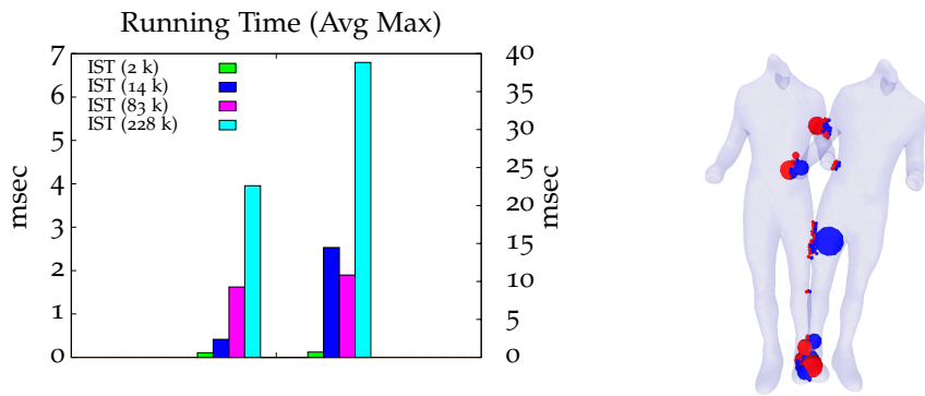
Figure 5.28: Time critical penetration volume computations in the torso scene (470k triangles). Left: average and maximum query time; The y axes are labeled differently.
