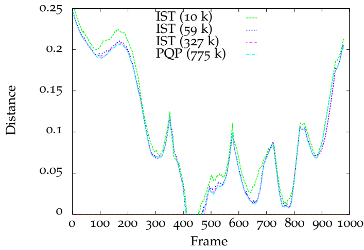
Figure 5.22: Distance per frame in the oil pump scene.
