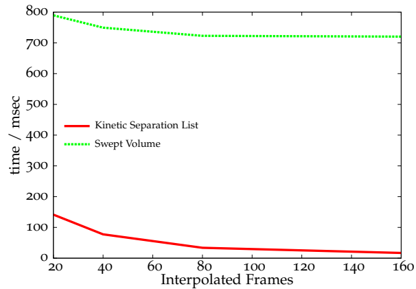
Figure 3.35: Male cloth animation scene: Total time, including updating and collision check, in the resolution of 49K triangles, depending on the number of interpolated frames in-between two key frames. Since the number of events only depends on the number of key frames and not on the number of interpolated frames, the average update time decreases if we increase the total number of frames.
