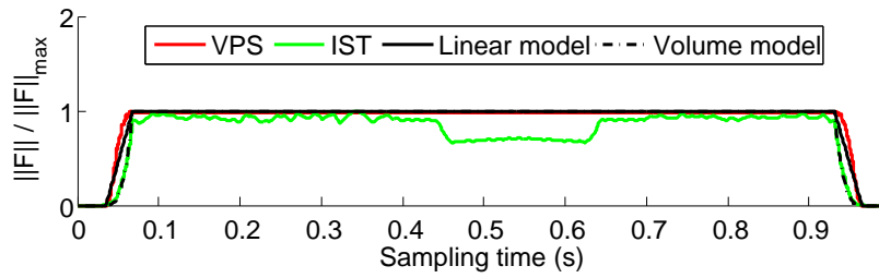
Figure 6.37: Forces in Scenario I.
