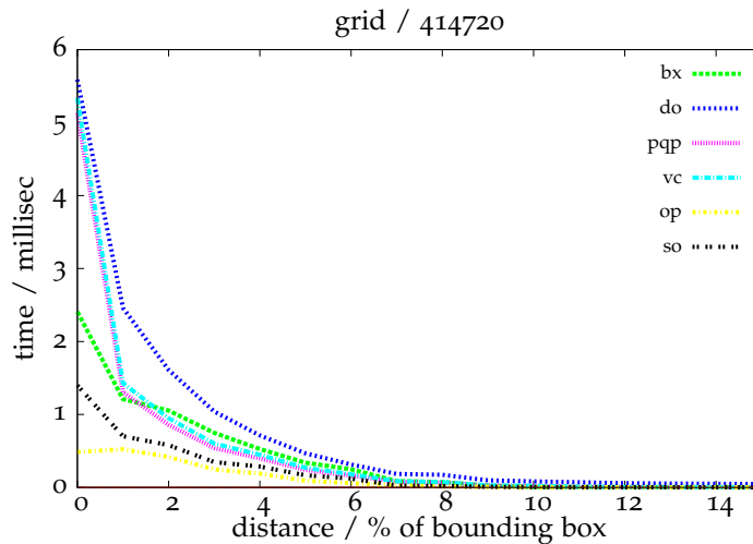
Figure 6.22: The results of the benchmark for the grid scene with 414 720 vertices. The notation is the same as in Figure 6.21
