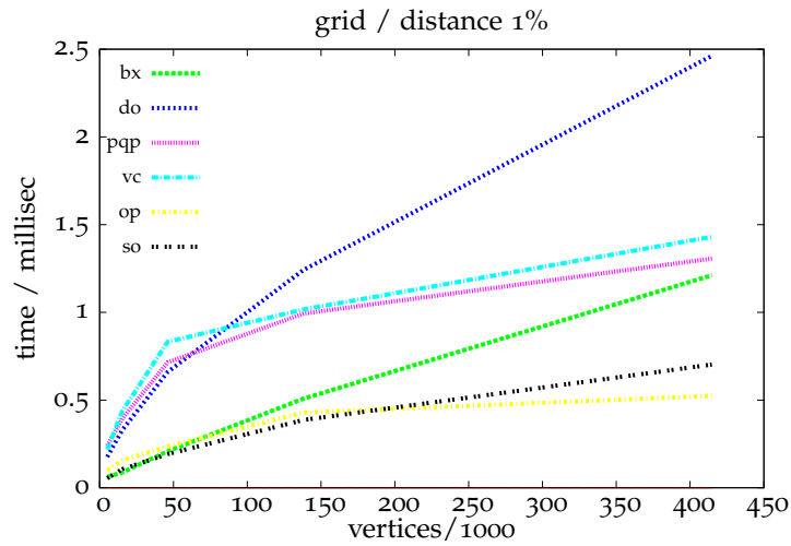
Figure 6.26: The results of the benchmark for the grid scene for a distance of 1% relative to the object size. The x -axis denotes the number of vertices divided by 1000. In contrast to the lustre scene (Figure 6.25) the running-time seems to increase in O(n \log n) for all algorithms.
