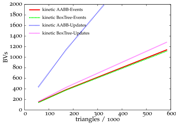
Figure 3.28: Catwalk scene: Average number of events and updates. The ratio seems to be nearly the same as in the tablecloth scene.
