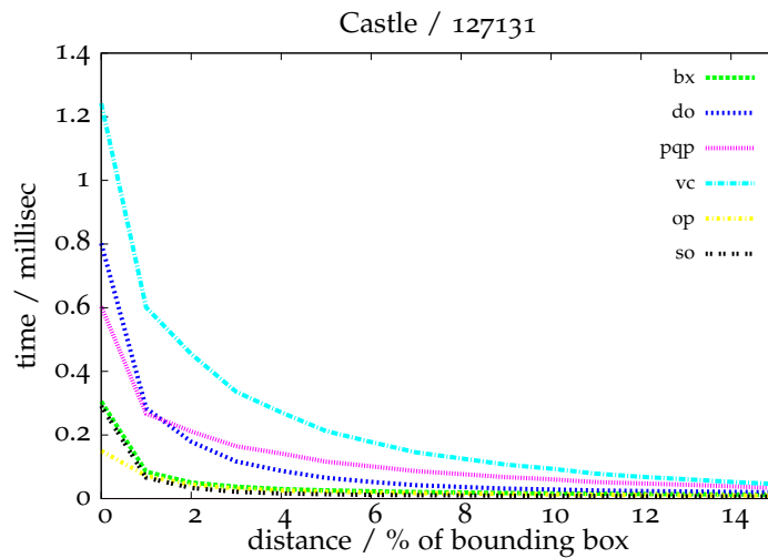
Figure 6.21: The results of the benchmark for the castle scenario in resolutions with 127 131 vertices. The x-axis denotes the relative distance between the objects, where 1.0 is the size of the object. Distance 0.0 means that the objects are almost touching but do not collide. The abbreviations for the libraries are as follows: bx=BoxTree, do=Dop-Tree, pqp=PQP, vc=V-Collide, op=Opcode, so=FreeSOLID. The ABB-based algorithms perform best in this kind of scenarios.
