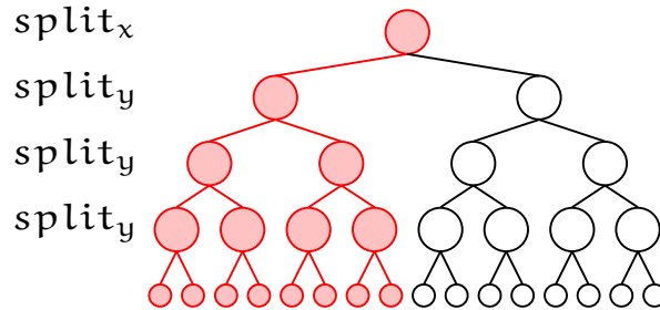
Figure 3.10: In the worst case, all levels have the same split axis, except of the root. If we want to compute a new event for the root, we have to traverse the whole tree.
