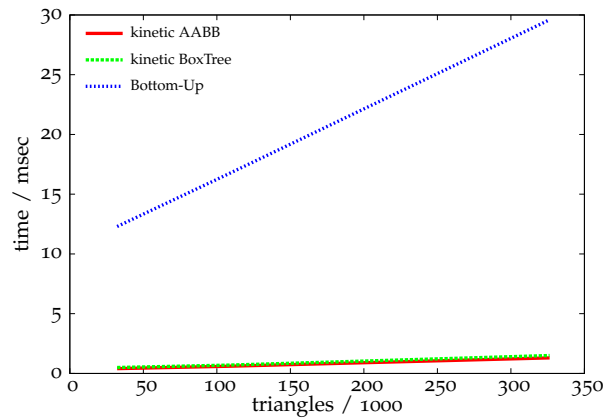
Figure 3.31: Male cloth animation scene: Average updating time. In this scene we have an overall gain of a factor about 10 for the kinetic AABB-Tree compared to the bottom-up-update.
