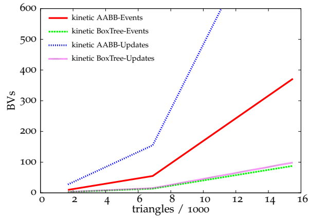
Figure 3.24: Tablecloth scene: Average number of events and updates per frame. The kinetic BoxTree has, as expected, has the smallest total number of events and the smallest number of total updates per event.
