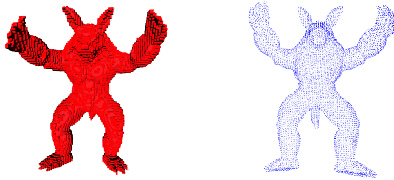
Figure 2.5: The Voxmap-Pointshell approach for 6 DOF haptic rendering uses two different data structures: A voxelization (left) and a point-sampling of the objects' surface (right).
