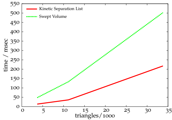
Figure 3.38: Swirling cloth scene: Time for updating and self collision check. Even in this worst case scenario for our algorithm, we have a gain of a factor about two for our kinetic data structure. This depends on the higher number of events in this scenario.
