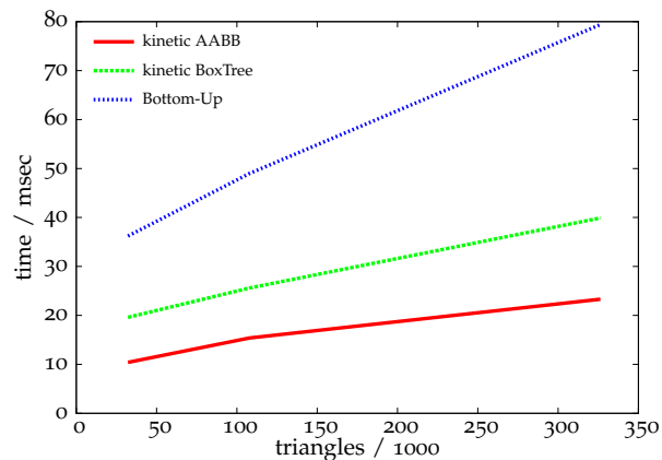
Figure 3.32: Male cloth animation scene: Total time, this means the time for updates and the proper check time.
