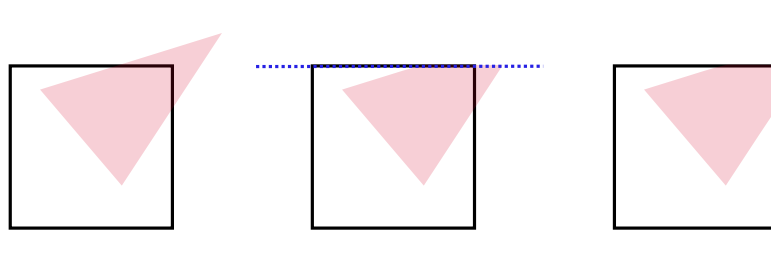
Figure 3.41: The red polygon is clipped consecutively against the spanning lines (blue) of the clip polygon (black).
