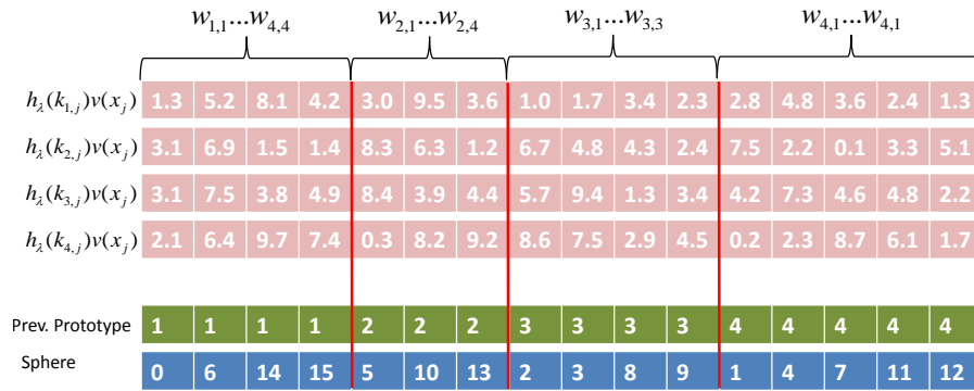
Figure 5.4: An example for the second level of the hierarchical BNG. According to Figure 5.3, each sphere (blue array) has been assigned to a prototype. We insert 16 new prototypes, w_{1,1}, \dots, w_{4,4} , 4 for each prototype w_1, \dots, w_4 from the previous level and compute the values that are required by BNG, e.g. h_\lambda(k_{ij})v(x_j) . Please note that we do not have to allocate new memory or copy any values from CPU to GPU. We can simply re-use the memory from the previous level because each sphere was assigned to exactly one prototype. Consequently, we get a constant memory consumption for each level.
