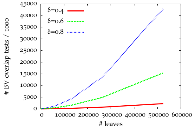
Figure 6.11: Same as Plot 6.9 with \alpha = 0.8
