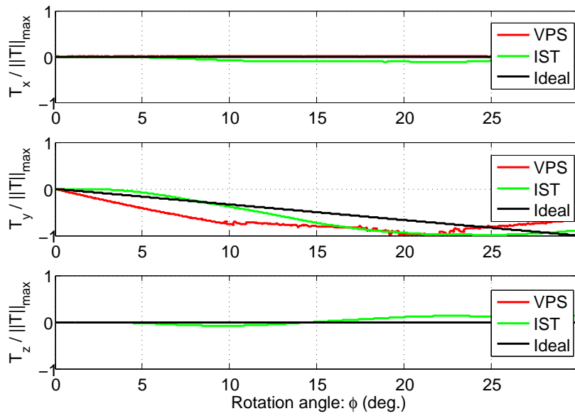
Figure 6.41: Torques in Scenario III.
