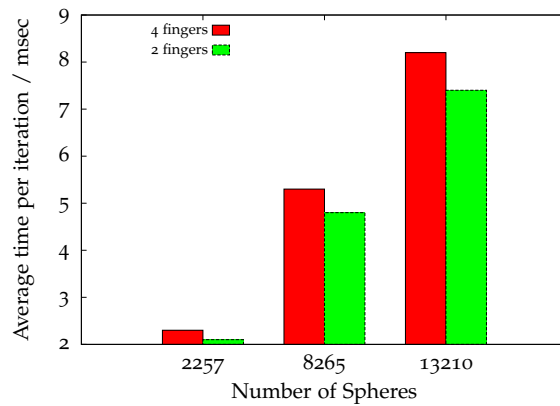
Figure 7.6: Average running-time during for two different movements of the virtual hand. In the first case (red) four fingers of the hand were moved simultaneously, while in the second case (green) only two fingers were moved.
